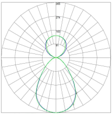
NORMALISED POLAR CURVE (DIRECT/INDIRECT)
